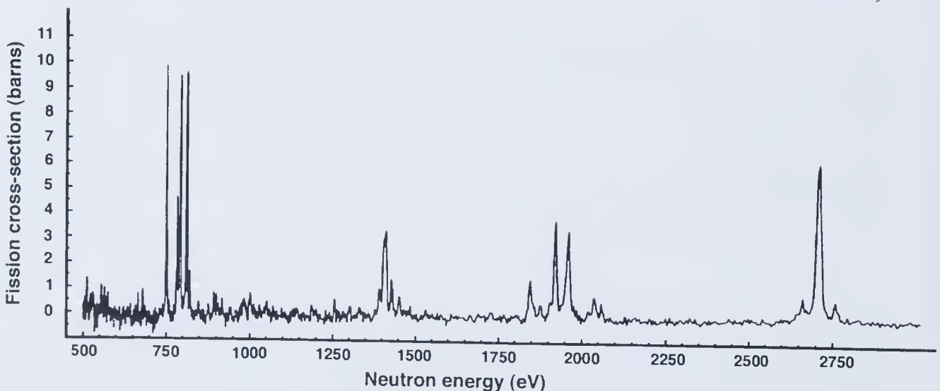
Figure 5. The neutron fission cross section of 240 Pu between 500 eV and 3000 eV (adapted from Migneco & Theobald 1968).
